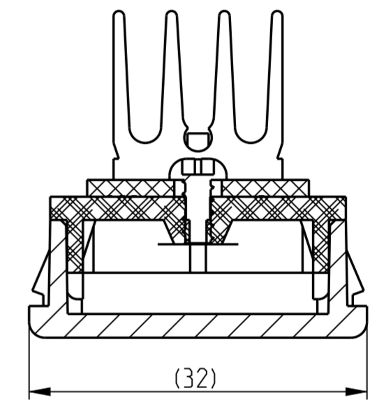
Section view A-A (2:1)
